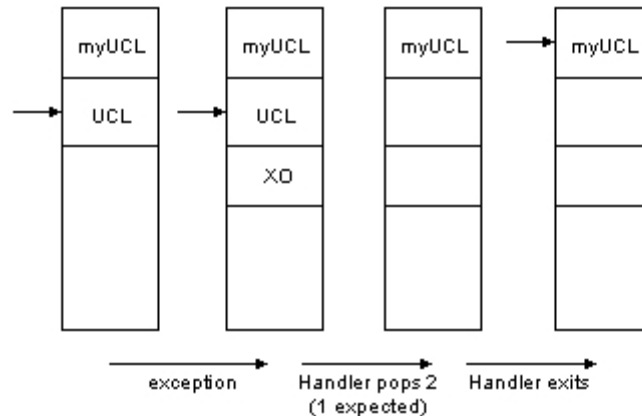
Figure 2: Stack depth invariance constraint violated in a malicious exception handler
